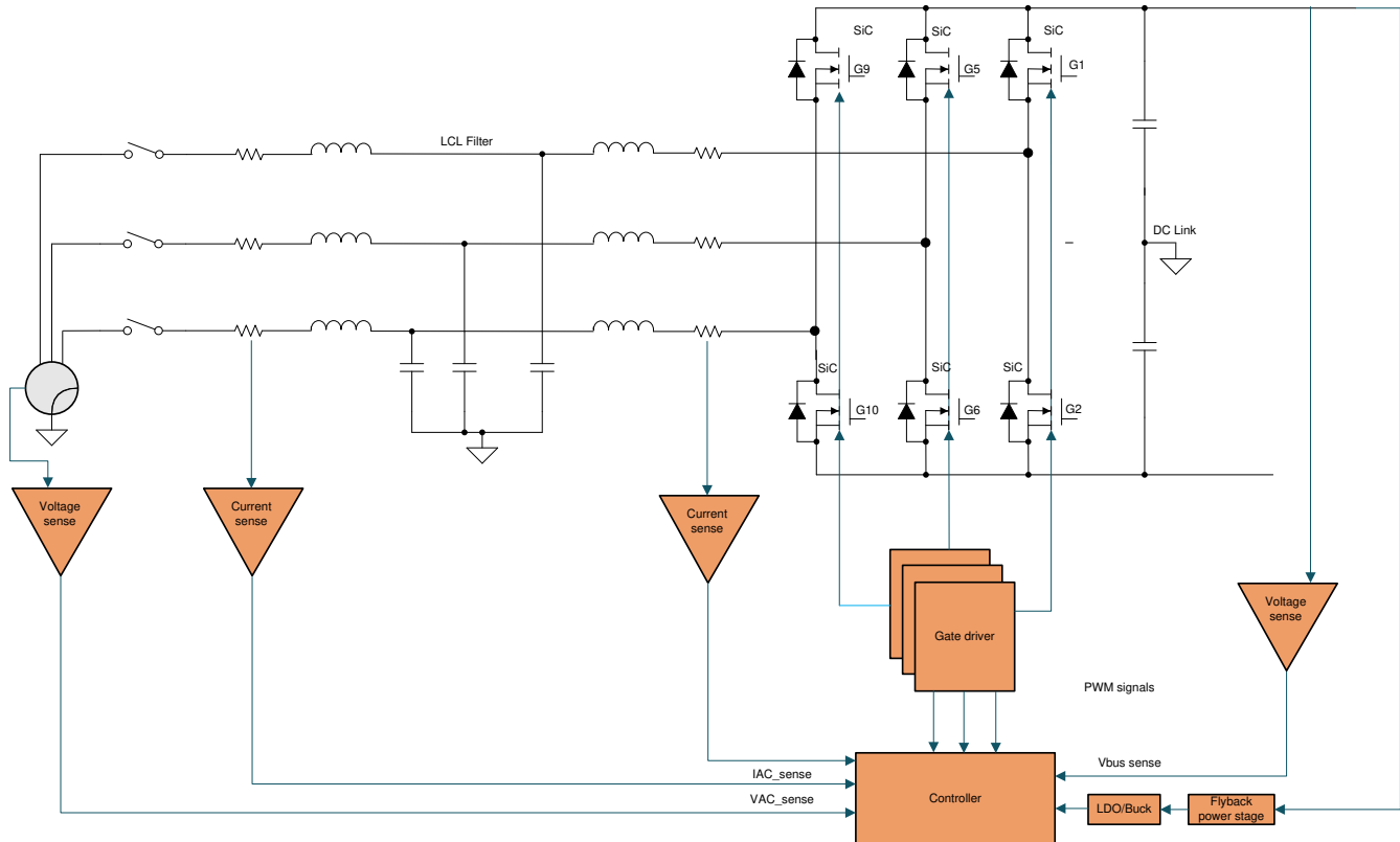
Figure 3-4. Two-level PFC
