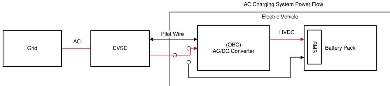
Figure 1-1. AC Charging Station
