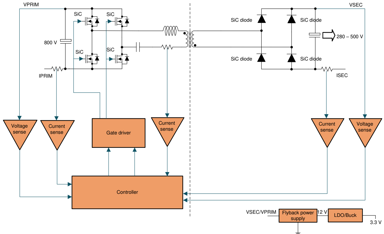
Figure 4-3. LLC Converter
